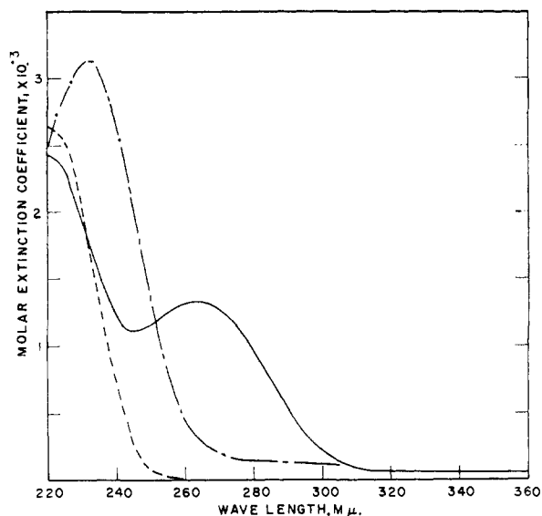
Fig. 2.—Absorption spectra for 1,4-disubstituted-5-iminotetrazoles and related compounds in water: —, 1,4-dimethyl-5-iminotetrazole hydrochloride; ---, 1-methyl-5-methylaminotetrazole; - · - ·, 1-methyl-5-aminotetrazole.
